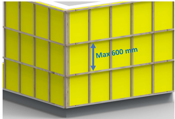
Battens and counter battens for vertical cladding
