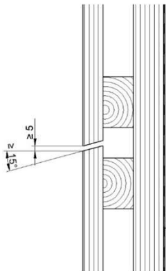
Joint without end matching
